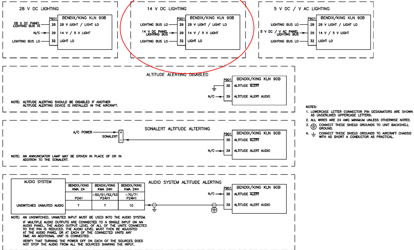
FIGURE 2-17 KLN 90B INTERCONNECT DRAWING (DWG. NO. 155-06021-0000, R-AC) (SHEET 9 OF 10)
