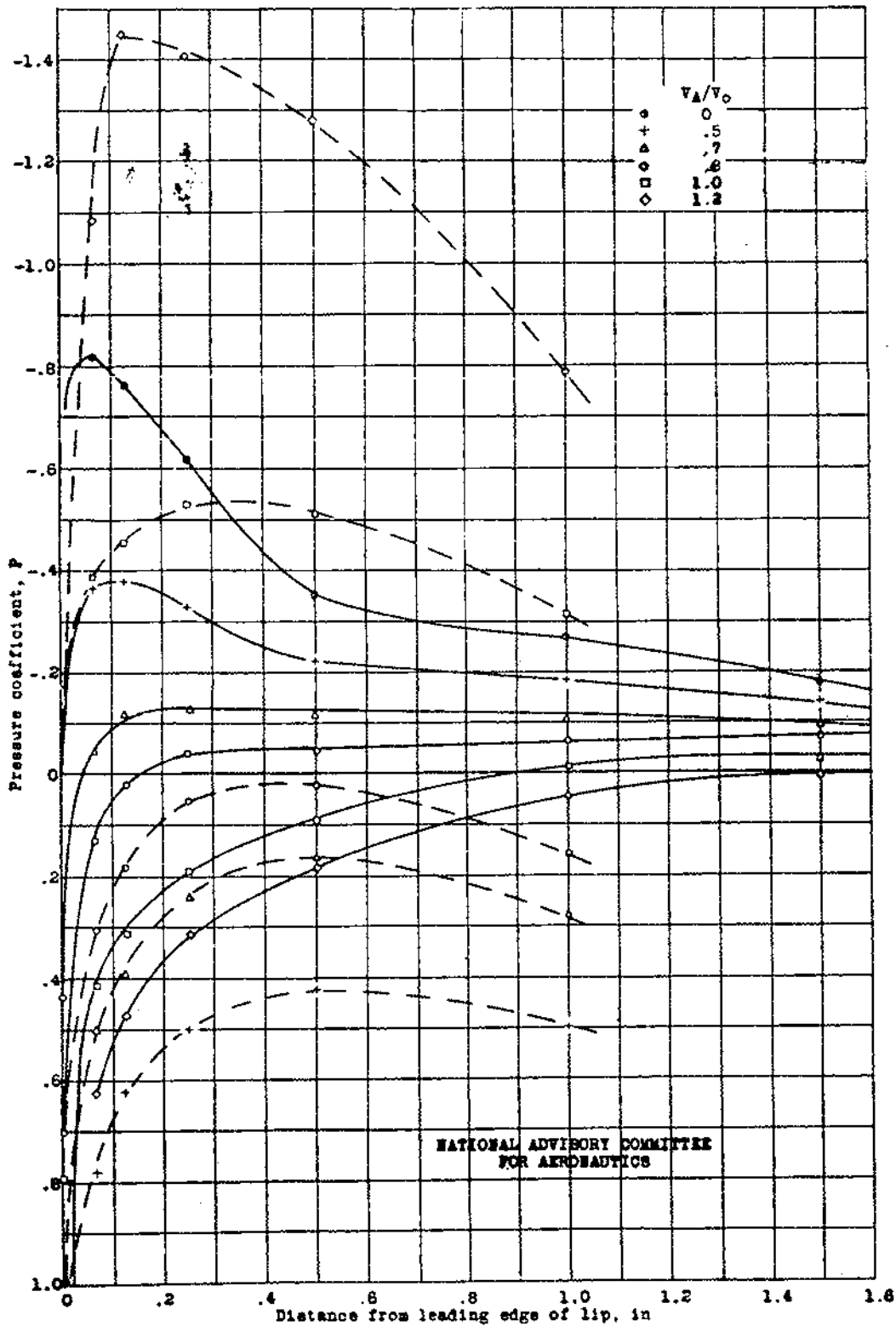
Figure 17.- Pressure distribution for various inlet-velocity ratios with lip 8 at -30^\circ incidence; 7^\circ ramp angle; boundary layer 1.
