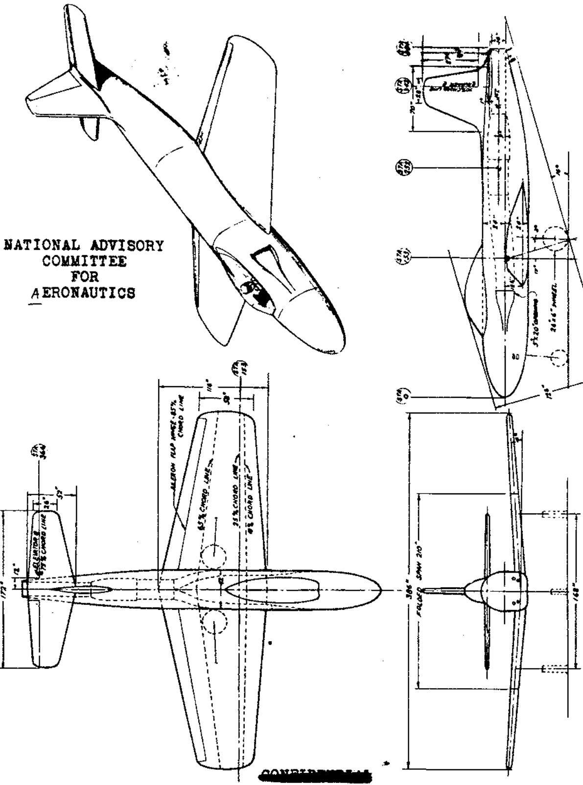
Figure 38.- Three-views of a high-speed fighter design.
