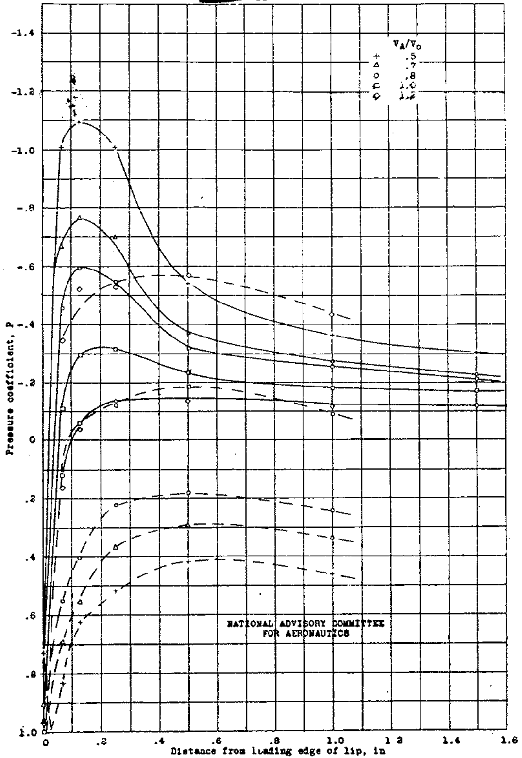
Figure 19.- Pressure distribution for various inlet-velocity ratios with lip 6 at zero incidence for a 5^\circ ramp angle; boundary layer 1.
