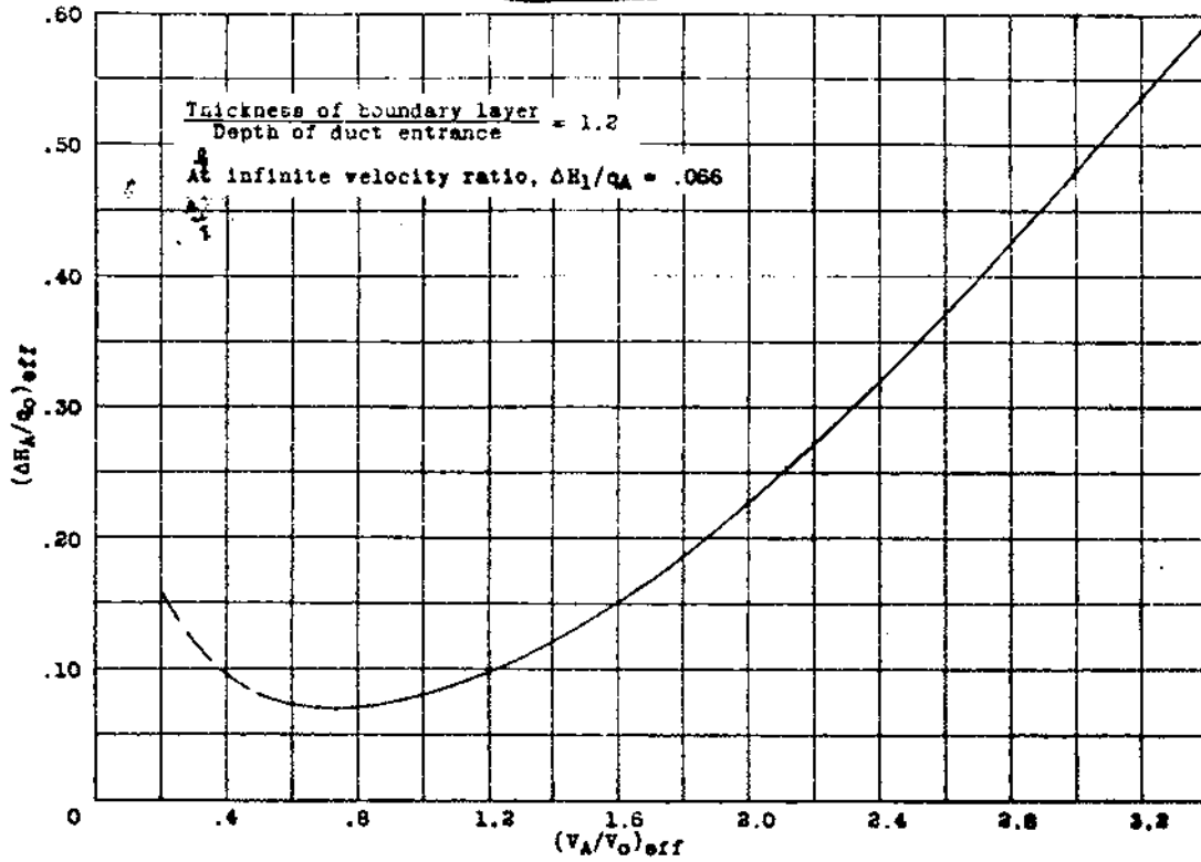
Figure 35.- Variation of effective entrance-dynamic-pressure losses with effective inlet-velocity ratio; extended deflectors; boundary layer 3.
