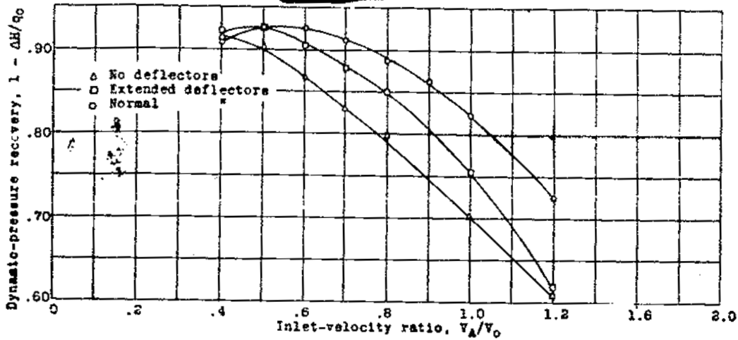
Figure 29.- Variation of dynamic-pressure recovery with inlet-velocity ratio for various deflector configurations. Submerged-duct installation on a .25-scale model of a fighter airplane. Pressure tubes mounted in entrance for comparison purposes only.
