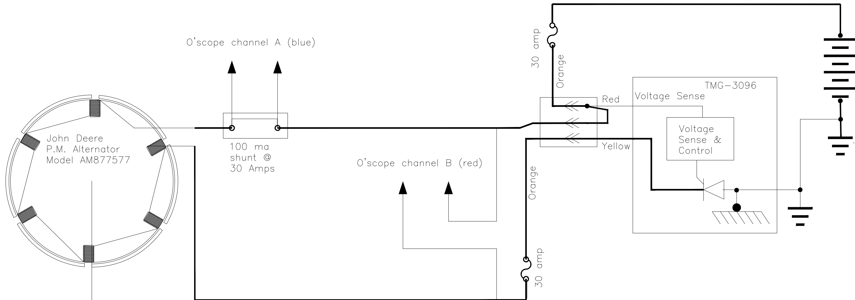
Revmaster R2300 regulator test Circuit
