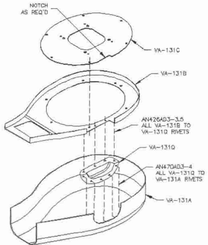
FIGURE 1: EXPLODED ISO VIEW
