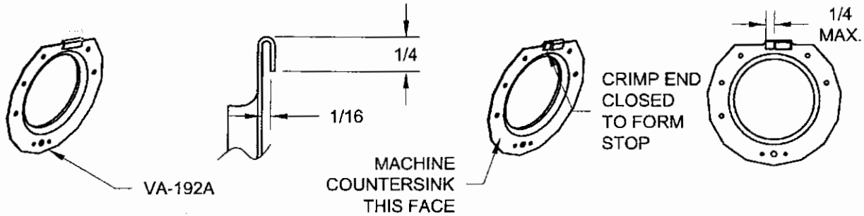
FIGURE 3: MAKING THE DOOR CATCH
