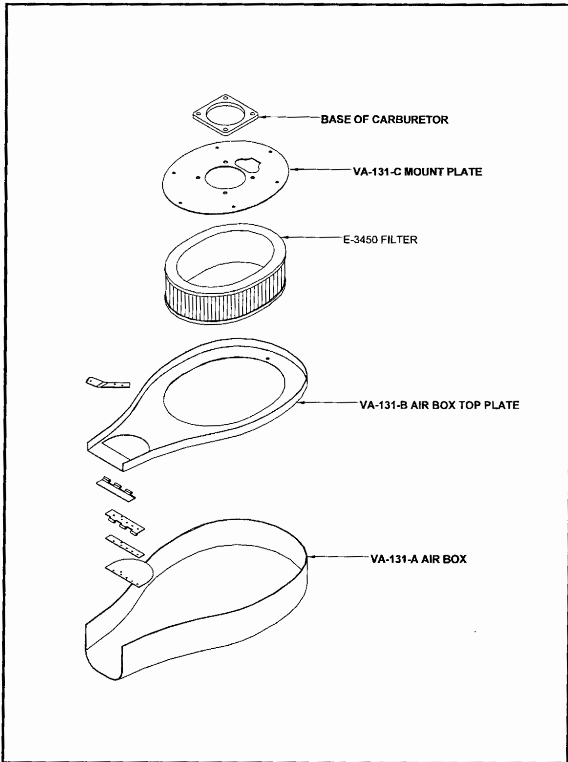
FIG. 1B O-360/540
