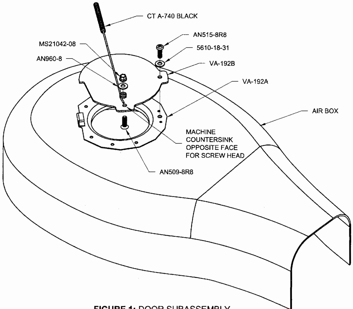
FIGURE 1: DOOR SUBASSEMBLY
