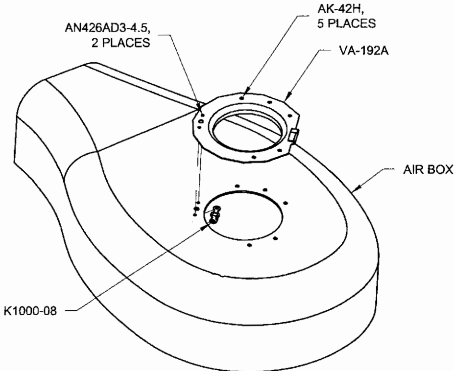
FIGURE 4: AIR INLET INSTALL
