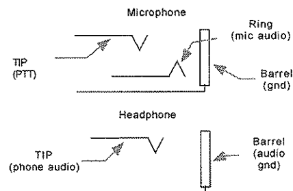
Monaural Headset Jack Details
