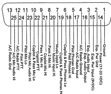
11922 Connector lay-out, viewed from rear
